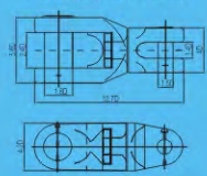
ANCHOR SWIVEL SHACKLE (a)= A.SW.S(a)(A型转环卸扣)
